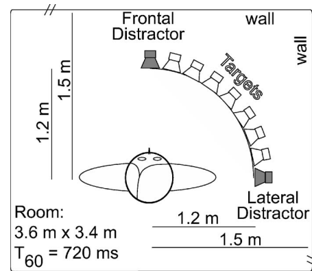
FIG. 1. Diagram of the orientation and location of the listener and the loudspeakers in the classroom used in Experiment 1. The same setup was used in the anechoic chamber in Experiment 2 although the (acoustically transparent) chamber walls were at different distances. In the figure the listener is facing the left-most loudspeaker and the targets are on his/her right. In half of runs, the listener was oriented to face the right-most loudspeaker and the targets were on his/her left.
