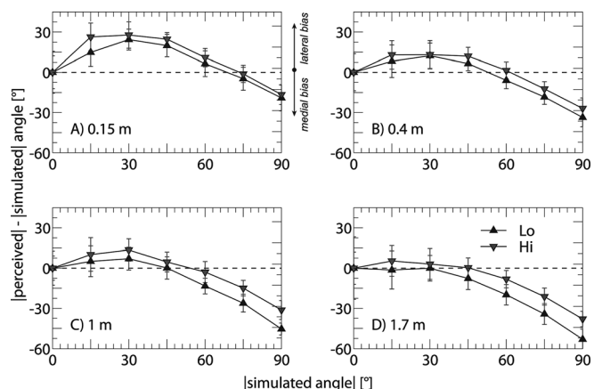
FIG. 2. Experiment 1: Mean signed response biases for Lo and Hi noise (black upward and gray downward triangles, respectively). Panels A–D each show one source distance. Error bars show one standard deviation across listeners.
